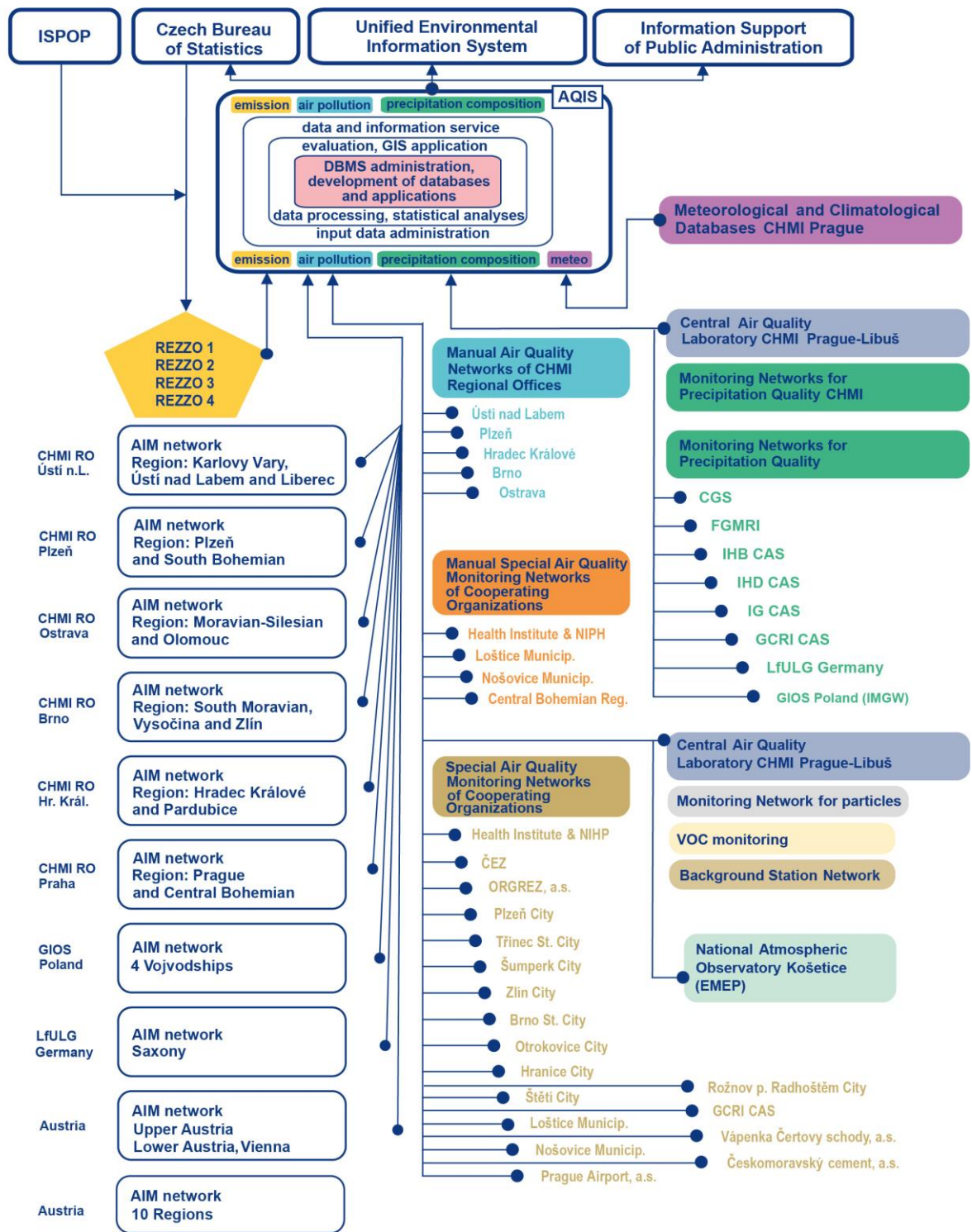
Fig. 1 Scheme of the AQIS links to data sources and cooperating systems in 2021
