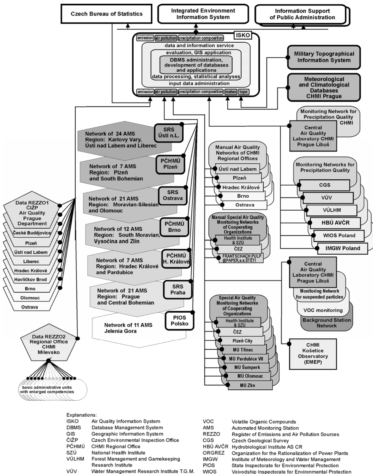
Fig. 1 Scheme of ISKO's links to data sources and cooperating systems in 2005
