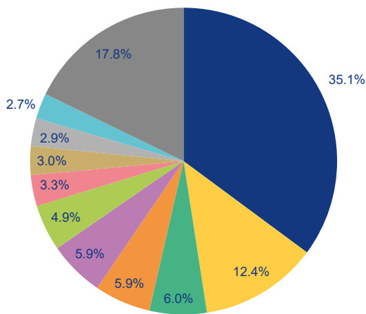
Fig. IV.9.1.2 Total emissions of VOC sorted out by NFR sectors, 2019
