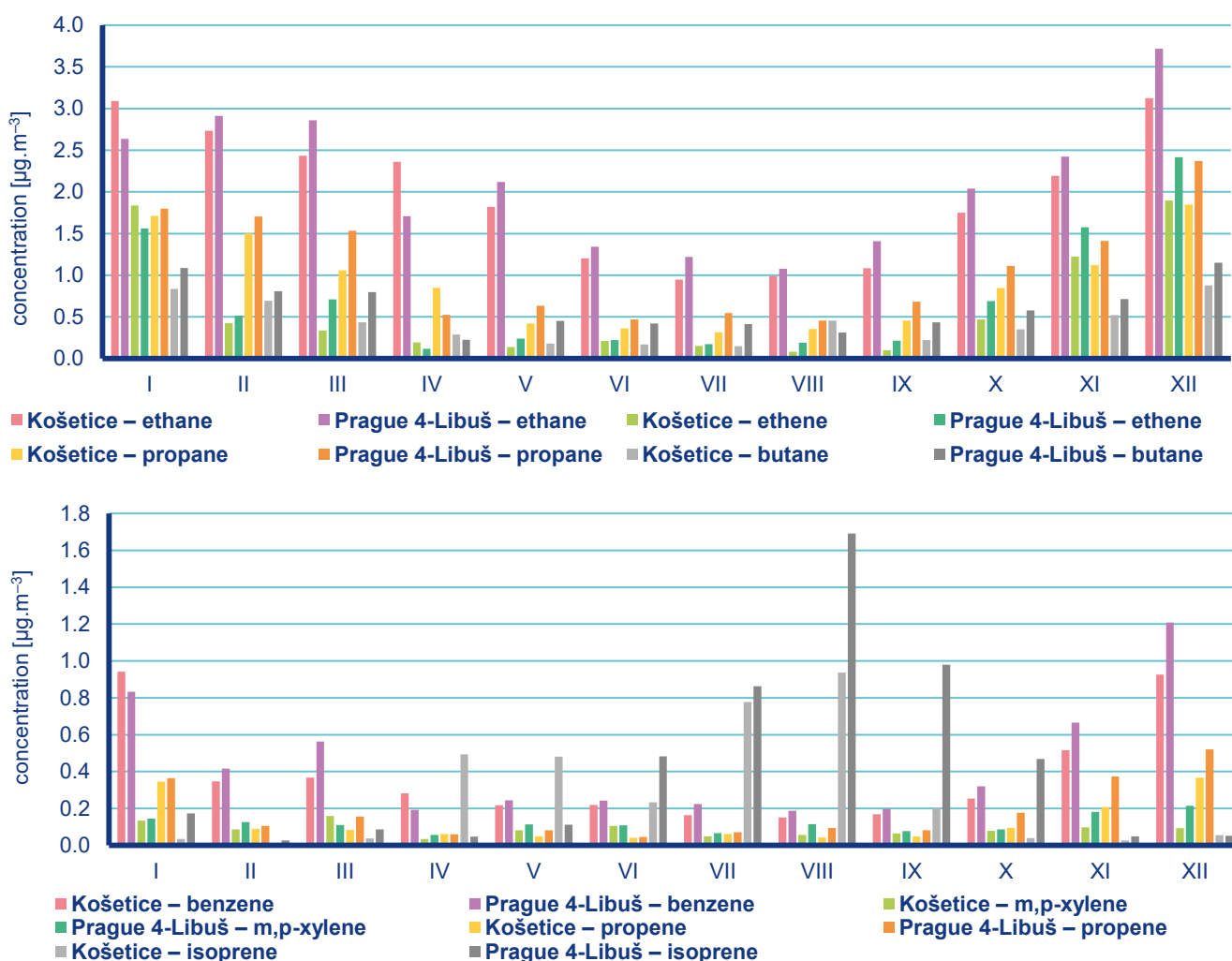
Fig. IV.9.1.1 Annual course of average monthly concentrations of VOC, 2020
