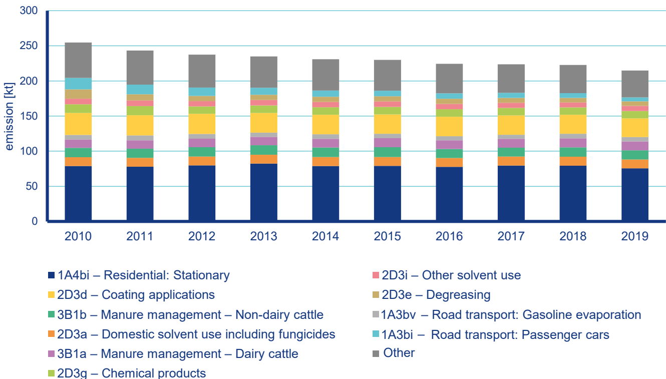
Fig. IV.9.1.3 VOC total emissions, 2010–2019
